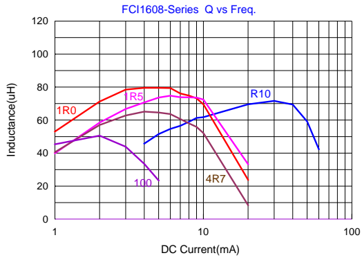
■ Q-Frequency Characteristics
