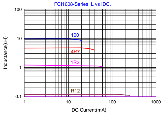
■ Inductance-Current
